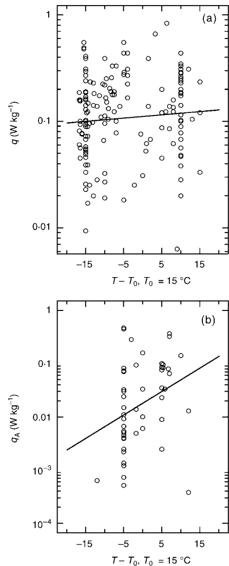
Fig. 5. (a) Temperature-independence of minimum life-supporting metabolic rates q ; \log_{10} q = a + b(T - T_0) , a = -0.91 \pm 0.03 (\pm 1 \text{ SE}) , b = 0.0046 \pm 0.0028 (\pm 1 \text{ SE}) , P = 0.10 , r^2 = 0.02 , n = 173 . (b) Temperature dependence of anoxic rates of energy dissipation q_A ; \log_{10} q_A = a + b(T - T_0) , a = -1.74 \pm 0.12 (\pm 1 \text{ SE}) , b = 0.044 \pm 0.019 (\pm 1 \text{ SE}) , P = 0.023 , r^2 = 0.097 , n = 53 .
