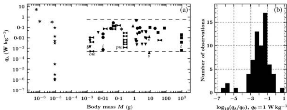
Fig. 3. Mass-specific rates q_A of energy dissipation by animals during various periods of anoxia. (a) Boxes, circles, triangles, up-down triangles and bow-ties denote vertebrates, arthropods (insects and crustaceans), gastropods, bivalves and worms, respectively. Asterisks denote the bivalve Crassostrea virginica developmental stages from larvae to adult organism and anoxia periods from 3 to 15 h at 22–25 °C (Widdows et al. 1989; Stickle et al. 1989). Stars denote embryos of Artemia franciscana during the following anoxia periods (counted downwards): 9 h, 6 days (Hand 1990), 1.5 h (Hontoria et al. 1993), 12 h, 1 month, 1.4, 2.5 and 5.6 years (Warner & Clegg 2001) at room temperature. Letters referring to groups of vertically arranged symbols denote the following species and anoxia periods (counted downwards): t turtle Chrysemys picta bellii , 0.5, 3, 10 and 84 days at 20, 15, 10 and 3 °C, respectively (Herbert & Jackson 1985); s snail Pila virens , 3 days of anoxia in the active hydrated state and 6 months of anoxic aestivation at 27 °C (Meenakshi 1957); pw priapulid worm Halicryptus spinulosus , 1, 2, 5, 10, 12 and 14 days at 10 °C (Oeschger et al. 1992); b bivalves Pisidium spp., 14, 100 and 140 days; ow oligochaete worm Potamothrix hammoniensis , 14, 61 and 134 days; i aquatic insect larvae Chironomus anthracinus (Diptera), 5, 15 and 25 days (Hamburger et al. 2000). Dashed lines are 95% CI of q -values for M > 1 mg assuming log-normal distribution. With one exception (see above), all values are for temperatures from 10 to 30 °C. (b) Frequency distribution of \log_{10} -transformed q_A values.
