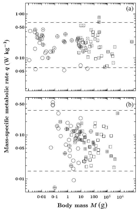
Fig. 1. Minimum life-supporting mass-specific metabolic rates q in various organisms. Boxes and circles denote vertebrates and invertebrates, respectively. Open symbols refer to temperatures \leq 5 °C, dotted symbols refer to temperatures > 5 °C and < 15 °C, symbols with a + refer to temperatures \geq 15 °C. Dashed lines denote 95% confidence intervals assuming a log-normal distribution of q -values. (a) Hibernating endotherms, arthropod sit-and-wait strategists, coldwater arthropods, i.e. groups I, II and III from Table 1, n = 80 species. (b) Coldwater fish and hibernating ectothermic vertebrates, aestivating vertebrates, coldwater non-arthropod invertebrates, aestivating non-arthropod invertebrates, i.e. groups IV, V, VI and VII from Table 1, n = 93 species.
