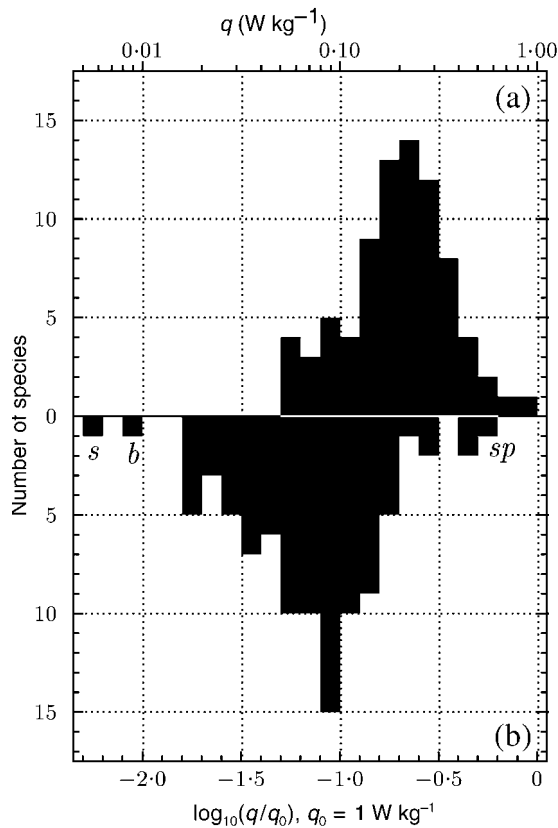
Fig. 2. Frequency distribution of \log_{10} -transformed minimum life-supporting mass-specific metabolic rates q in: (a) endotherms and arthropods (Groups I–III from Table 1) and (b) ectothermic vertebrates and non-arthropod invertebrates (Groups IV–VII from Table 1). Outliers: s aestivating Tanzanian snail Bulinus nasutus (shell-free mass 0.1 g, 24 °C); b Arctic bivalve Astarte montagui (ash-free dry mass 0.6 g, 0 °C); sp coldwater sponges from the Norwegian Sea (ash-free dry mass 10–20 mg, –0.5 °C).
