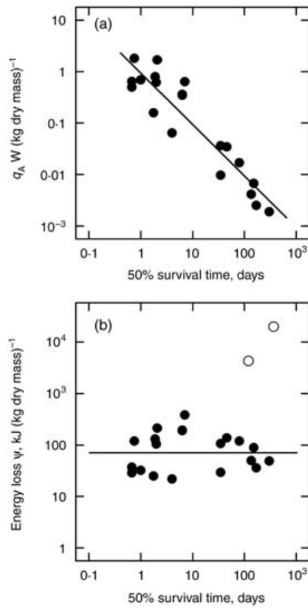
Fig. 4. Metabolic rate, energy loss and survival time in anoxia. (a) Mass-specific rates q_A of energy dissipation by organisms capable of surviving more than half a day of anoxia. Regression line \log_{10} q_A (\text{W kg}^{-1}) = -0.041 - 1.0 \log_{10} \text{LT}_{50} (\text{days}) , where \text{LT}_{50} is the 50% survival time ( P < 10^{-5} , r^2 = 0.86 , n = 20 ). (b) Filled circles: energy loss \psi (eqn 2) during anoxia; it is independent of survival time; regression \log_{10} \Psi = a + b \log_{10} \text{LT}_{50} gave a = 1.85 \pm 0.12 (\pm 1 \text{ SE}) , b = 0.02 \pm 0.09 , P = 0.85 , r^2 = 0.002 . Open circles: normoxic energy losses of bears during hibernation and ticks during prolonged starvation, see text for details.
